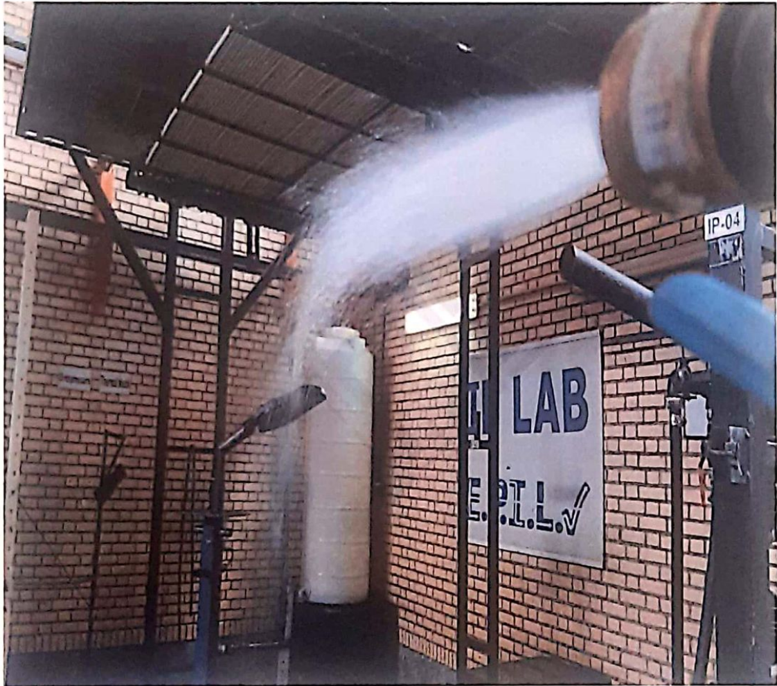
Figure 3: EUT under IPX6
