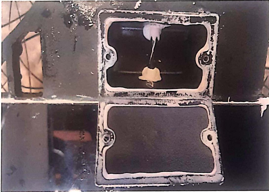
Figure 4: EUT after IPX6
